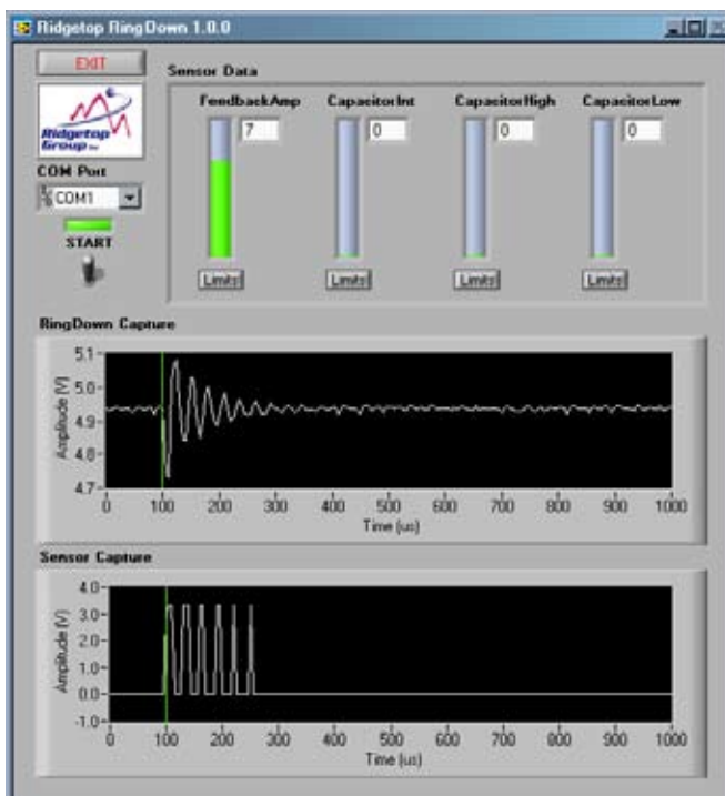
Example Interface for RingDown™ Power Prognostics
