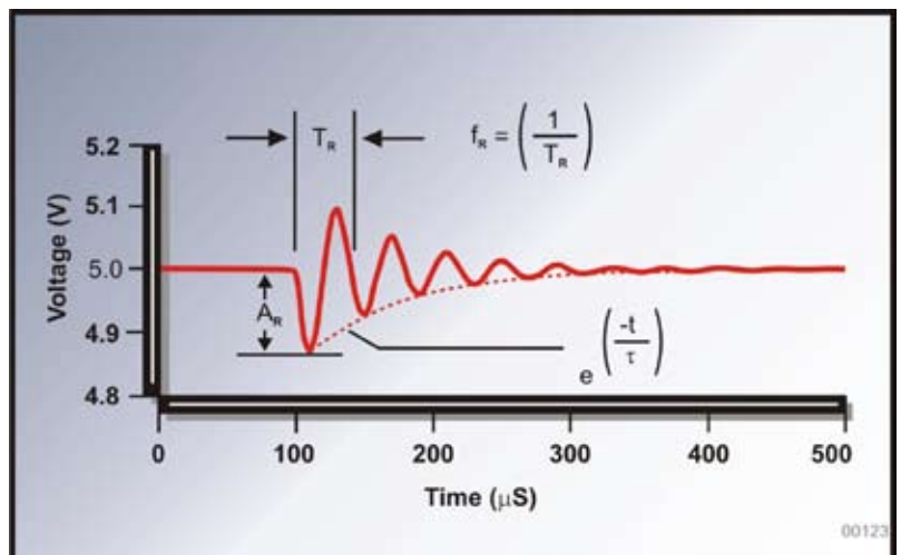
Damped Sinusoid Response or "Ringing" Signal in Response to a Load Change
